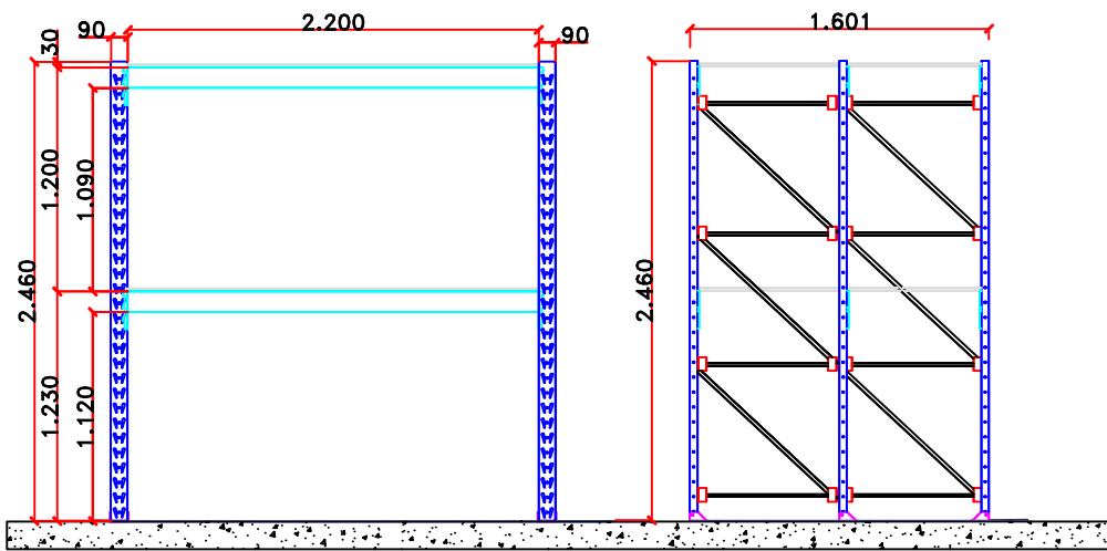
VISTA FRONTAL
