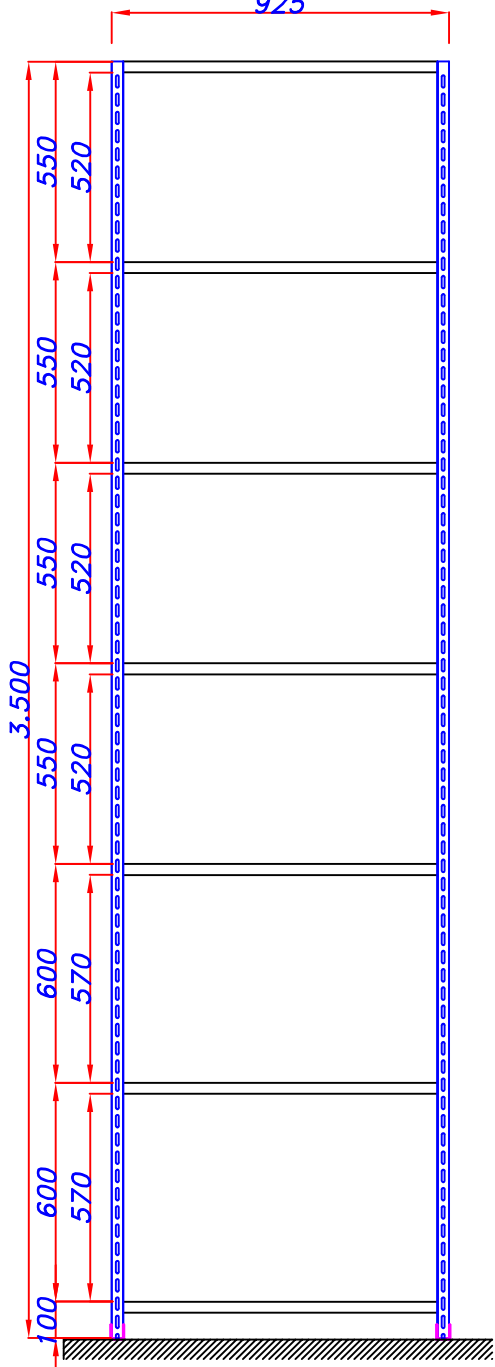
VISTA FRONTAL
